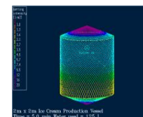
Spray Pattern Graphic
